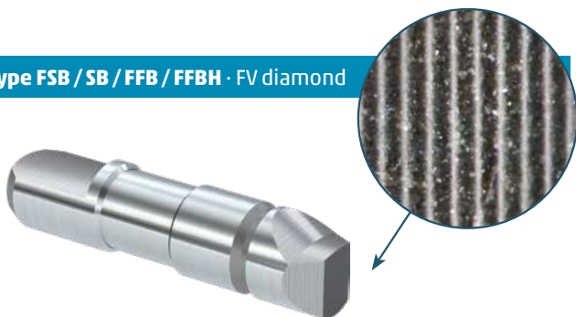
Technical data – type FSB / SB / FFB / FFBH · FV diamond
